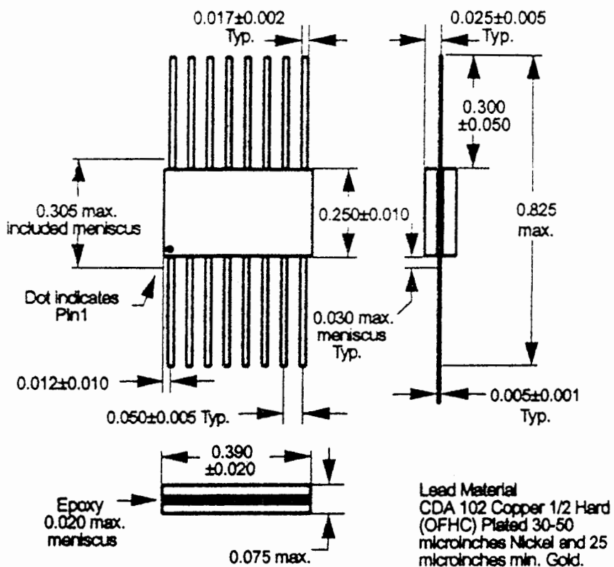
Figure 1. Package Outline.
